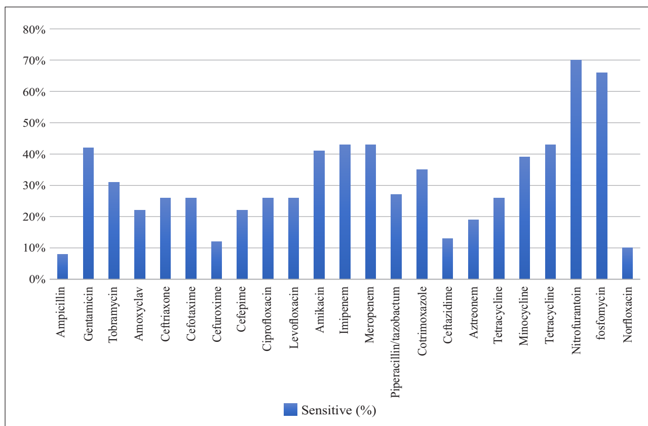
Figure 1: Antibiotic sensitive profile of Enterobacteriaceae (n=119)
