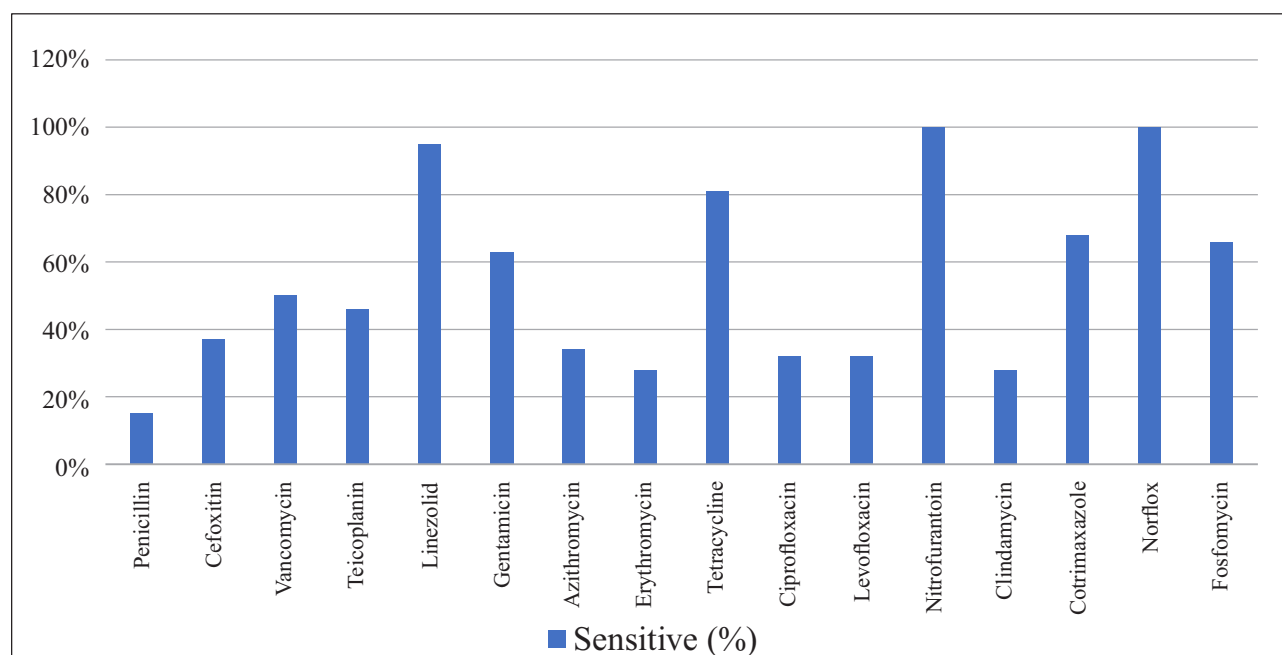
Figure 4: Antibiotic sensitive pattern of Staphylococcus aureus and CoNS (n=45)
