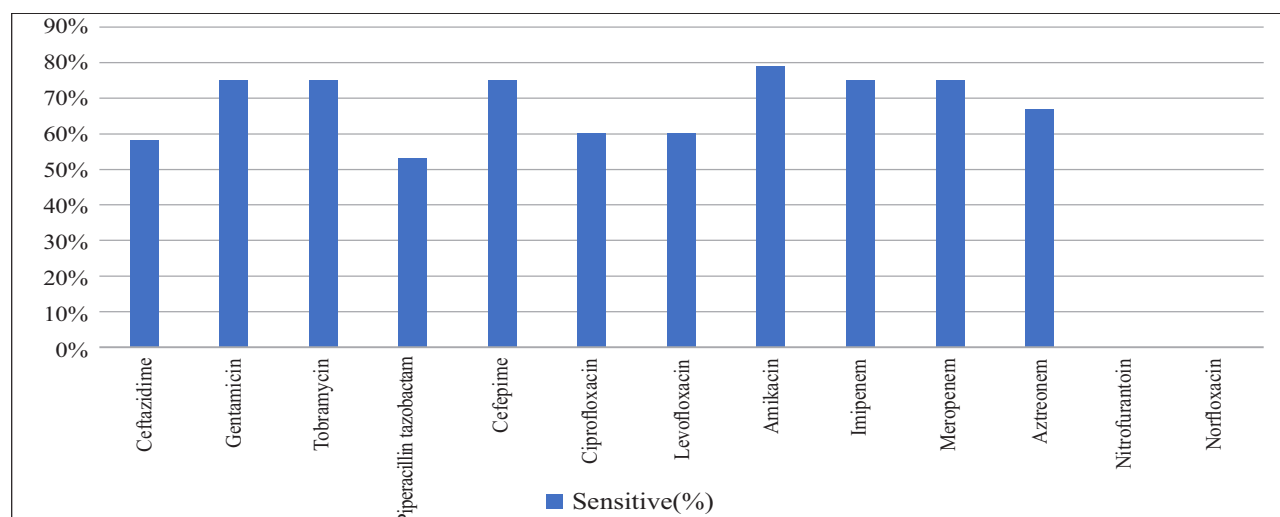
Figure 3: Antibiotic sensitive pattern of Pseudomonas aeruginosa (n=28)
