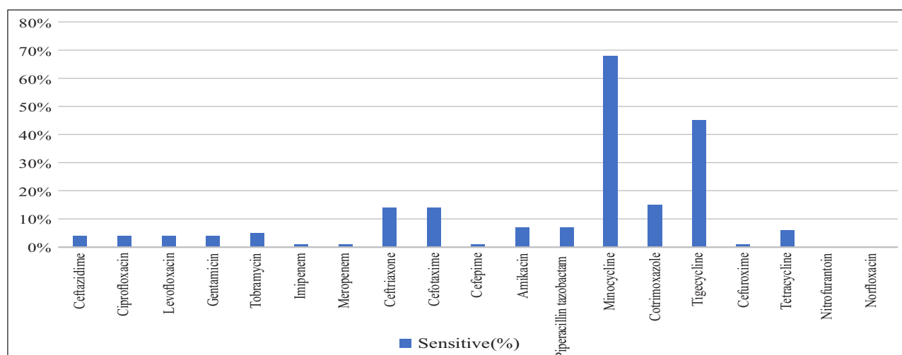
Figure 2: Antibiotic sensitive pattern of Acinetobacter spp. (n=65)
