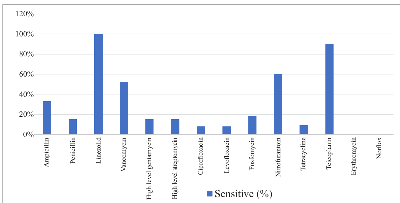
Figure 5: Antibiotic sensitive pattern of Enterococcus spp. (n=28)
