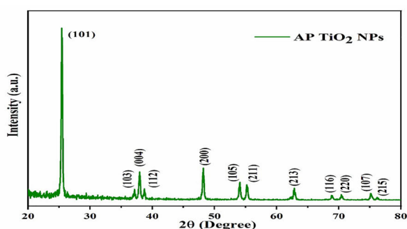
Figure 4: XRD pattern of titanium dioxide nanoparticles (APTiO 2 NPs) produced from aqueous extract of Alternanthera philoxeroides whole plant
