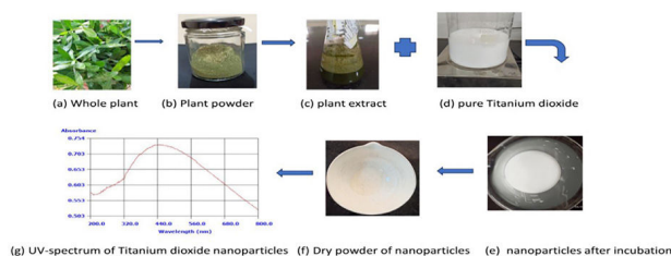
Figure 1: Green synthesis methods of titanium Dioxide nanoparticles using Alternanthera Philoxeroides
