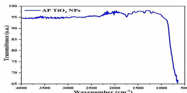
Figure 3: FTIR result of titanium dioxide nanoparticles using Alternanthera Philoxeroides
