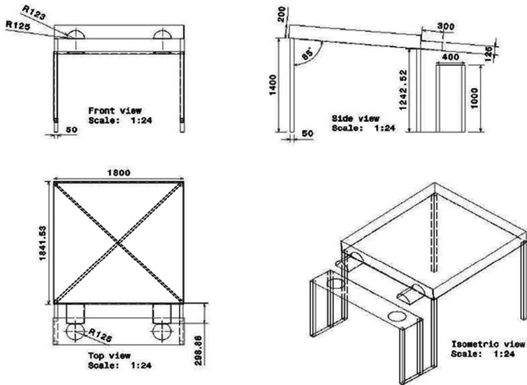
Fig. 8: Proposed Table for collecting and releasing concrete
