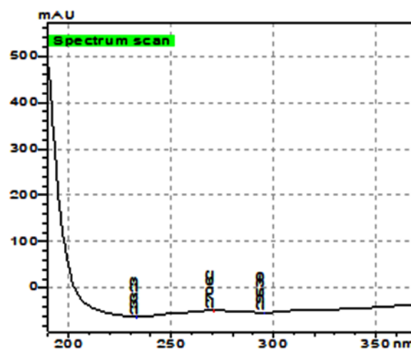
Fig. 2: HPLC Scan Spectrum for Cefotaxime sodium
