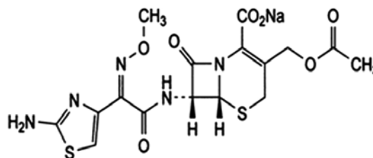
Fig. 1: Structure for Cefotaxime sodium
