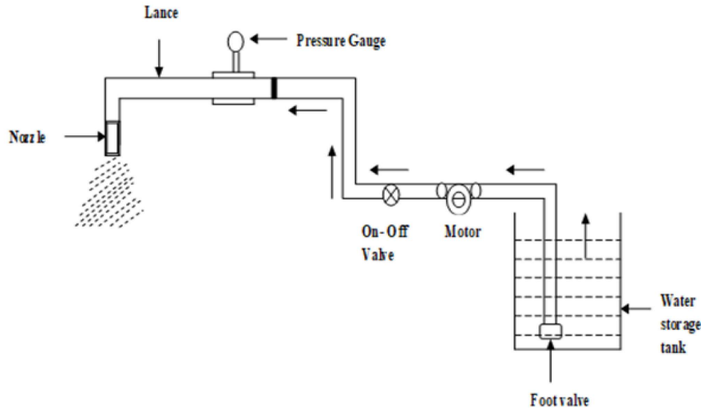
Fig. 1: Rainfall simulator
