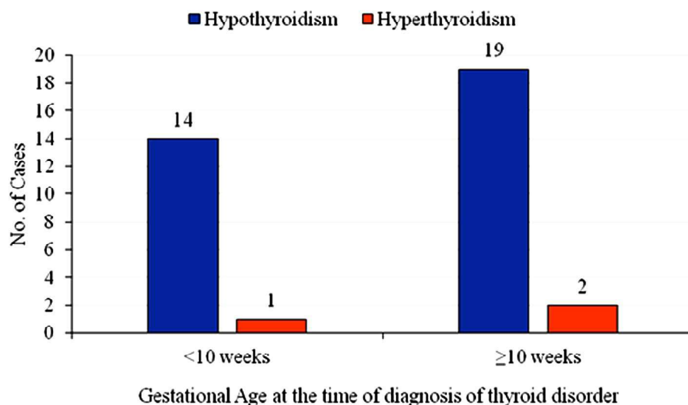
Fig. 2: Distribution of women according to the gestational age at the time of diagnosis of thyroid disorder
