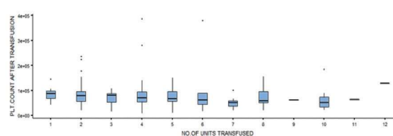
Fig. 2: Box plot representing platelet count after transfusion
