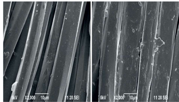
Fig. 6: SEM images of untreated and treated polycotton fabric
