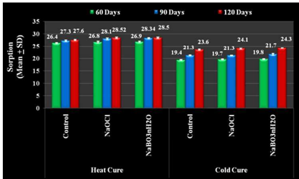
Graph 5: Sorption
