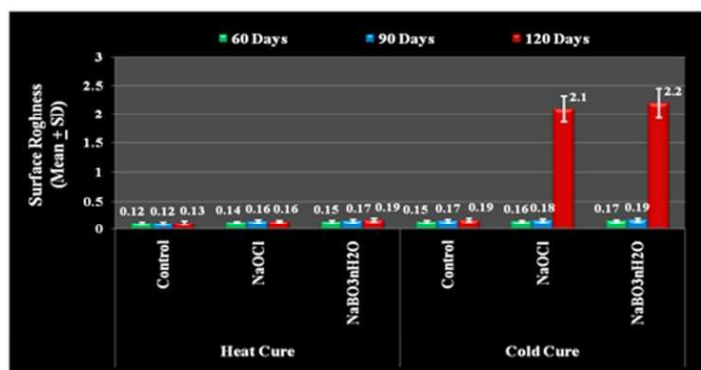
Graph 1: Surface roughness
