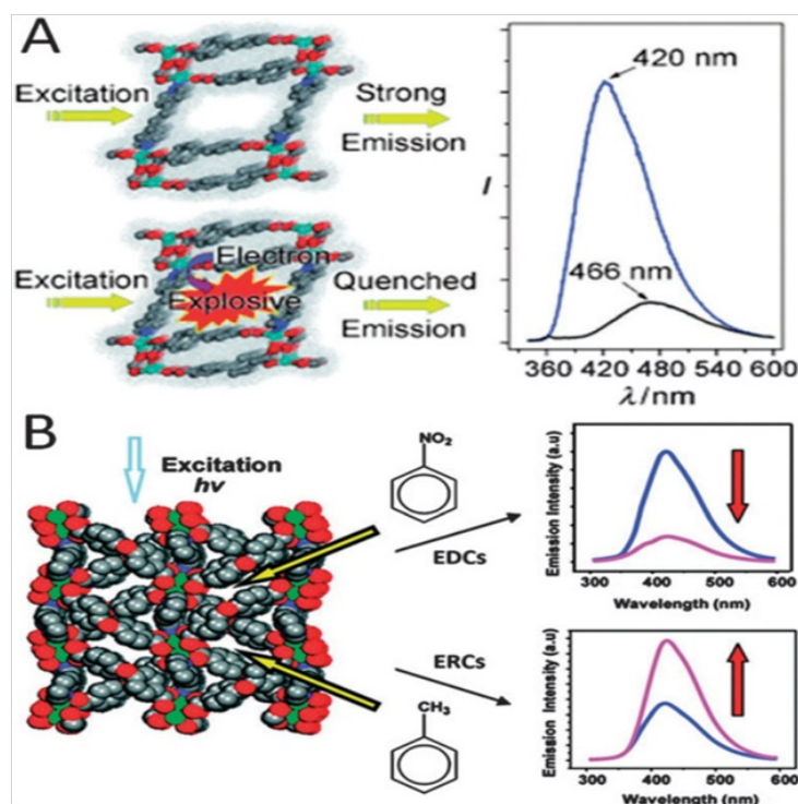
Figure 4: A highly luminescent microporous metal-organic framework, [Zn_2(bpdc)_2(bpee)] ( bpdc = 4,4\text{-biphenyldicarboxylate} ; bpee = 1,2\text{-bipyridylethene} ), capable of very fast detection of the vapors of nitroexplosives and the fluorescence spectra before and after exposure to DNMB vapor for 10 s. (B) A highly luminescent 3D microporous MOF, [Zn_2(oba)_2(bpy)] DMA, demonstrates unique selectivity for the detection of electron-deficient explosives (EDCs) and electron-rich aromatics (ERCs) via a fluorescence quenching and enhancement mechanism.
