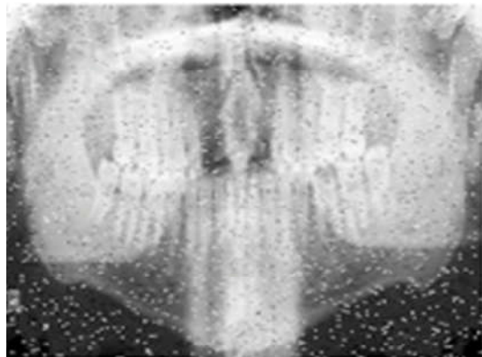
Fig. 2.10: Noisy image
