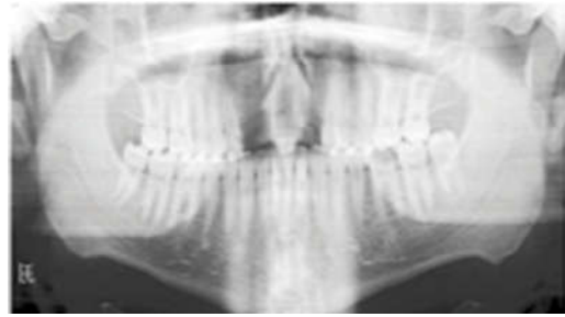
Fig. 2.7: Input image
