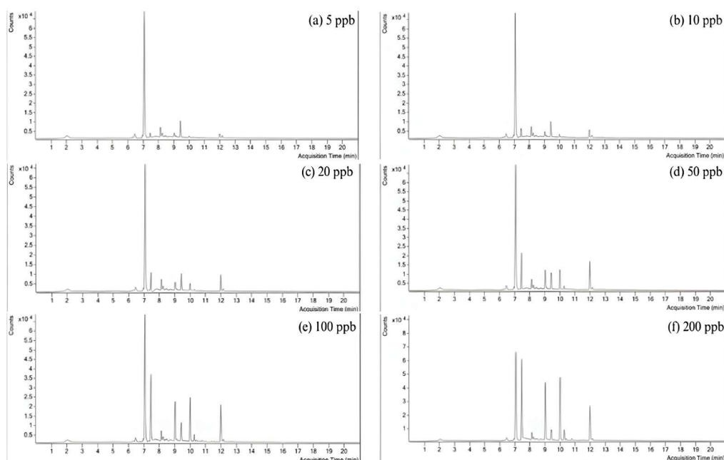
Fig. 3: LC-MS/MS Chromatogram for LMG, OXC, VA and TPM at concentrations (a) 5 ppb, (b) 10 ppb, (c) 20 ppb, (d) 50 ppb, (e) 100 ppb and (f) 200 ppb in biological matrix
