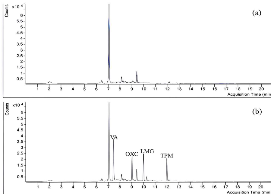
Fig. 1: Chromatogram of (a) Blank Matrix sample, (b) Spiked matrix with selected ACDs at 100 ppb
