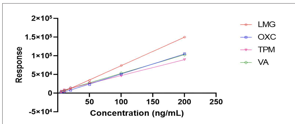
Fig. 2: Calibration curve of all the 4 drugs
