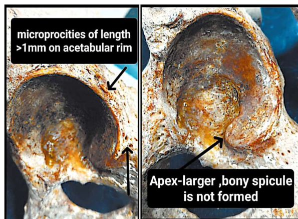
Figure 5.3: Acetabular Rim Porosity
