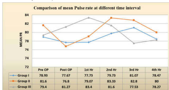
Fig 2: Mean heart rate in study subjects in the three groups at different time intervals.
