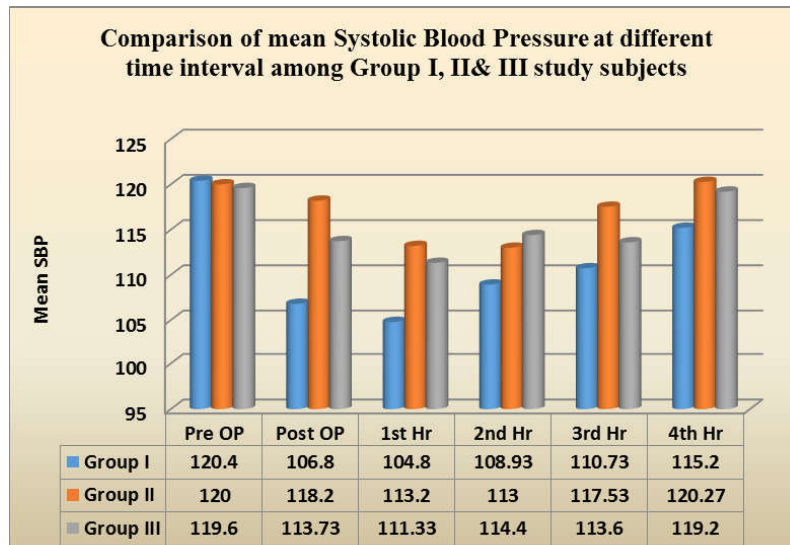
Fig 3: Mean systolic blood pressure in study subjects in the three groups at different time intervals.
